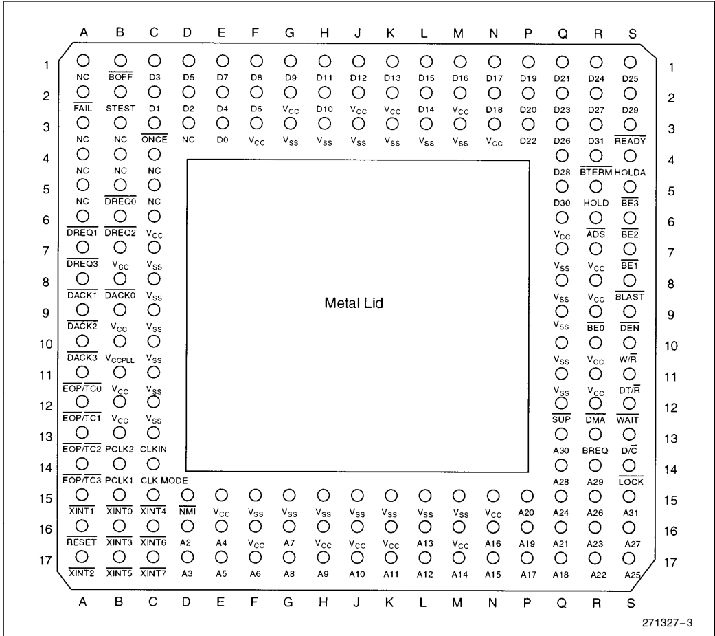
Figure 3. 80960CA PGA Pinout—View Lid from Bottom (Pins Facing Up)
