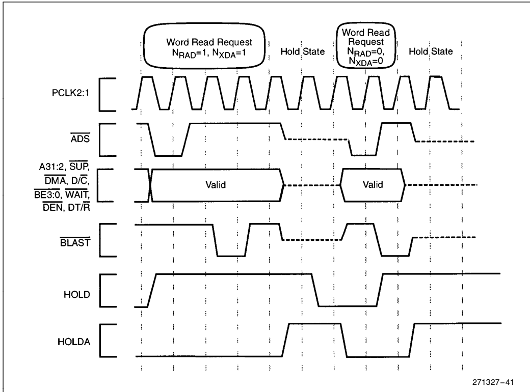
Figure 41. HOLD Functional Timing
