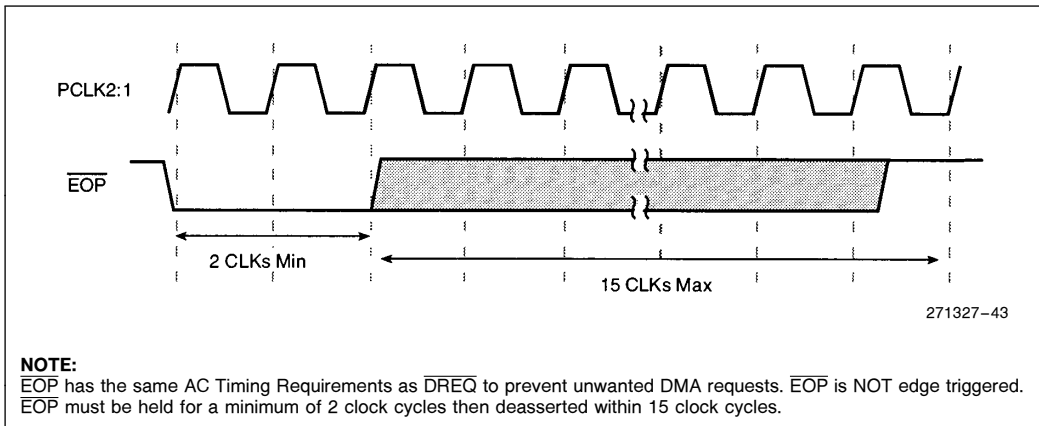
Figure 43. \overline{EOP} Functional Timing
