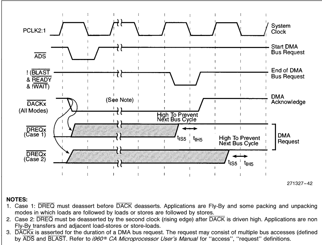
Figure 42. \overline{DREQ} and \overline{DACK} Functional Timing
