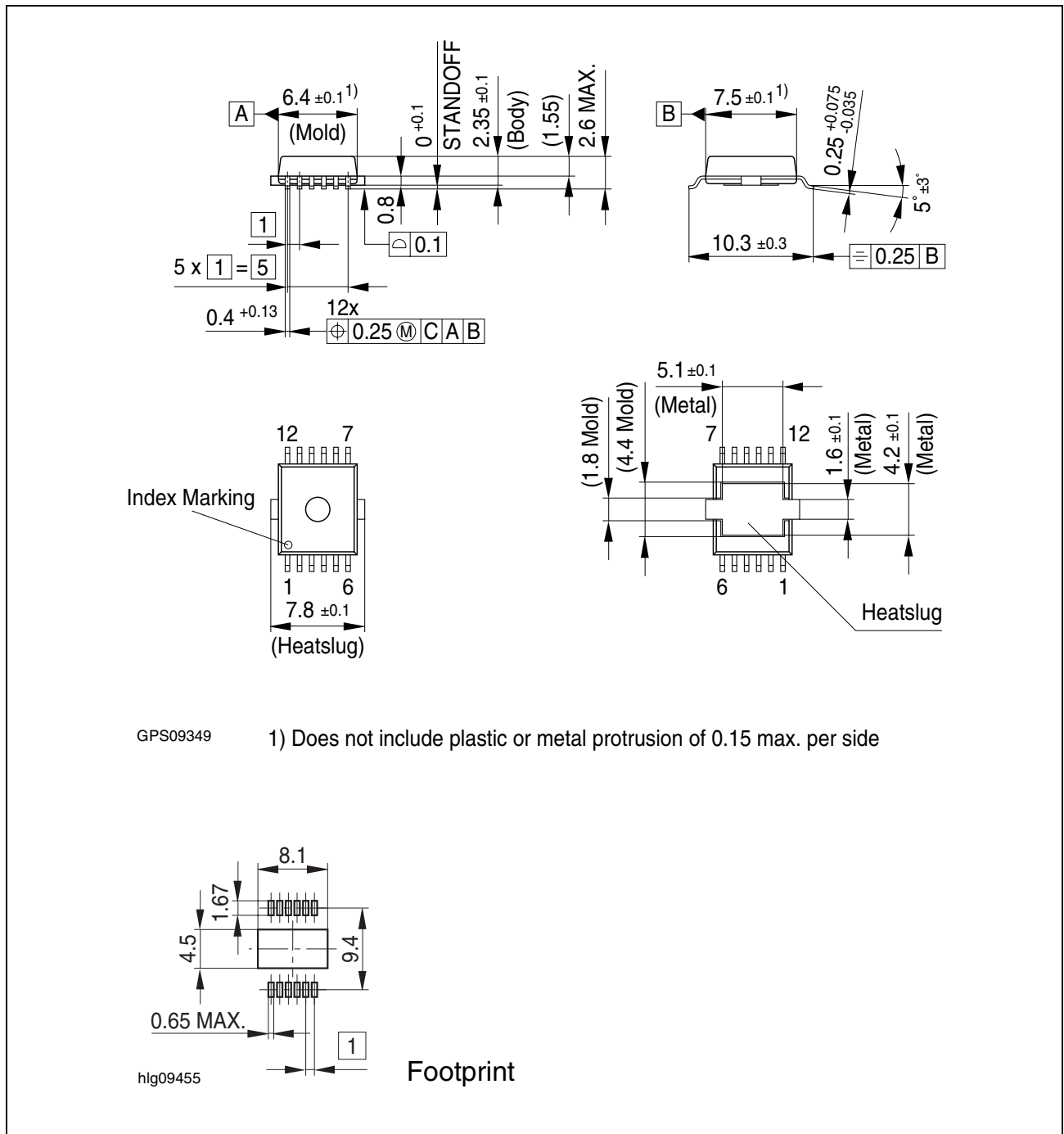
Figure 4 P-DSO-12-4 (Plastic Dual Small Outline)
