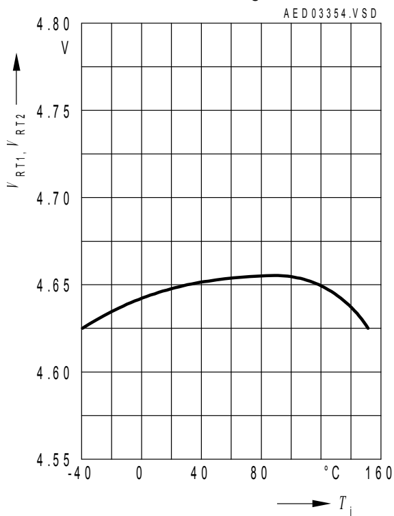
Reset Thresholds V_{RT1} , V_{RT2} versus Junction Temperature T_j
