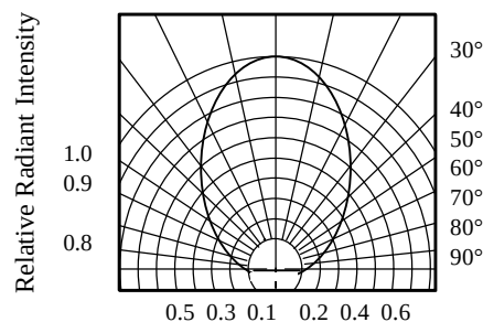
FIG.5 RADIATION DIAGRAM
