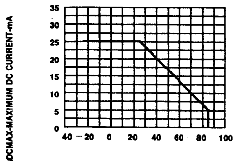
T A AMBIENT TEMPERATURE °C Fig.4 MAXIMUM ALLOWABLE DC CURRENT PER SEGMENT CS. A FUNCTION OF AMBIENT TEMPERATURE.
