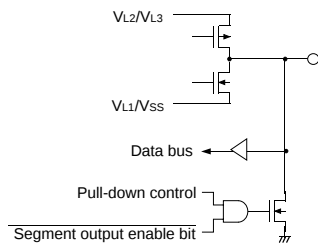
(3) Ports P30–P37
