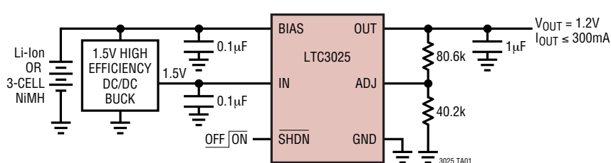
1.2V Output Voltage from 1.5V Input Supply
