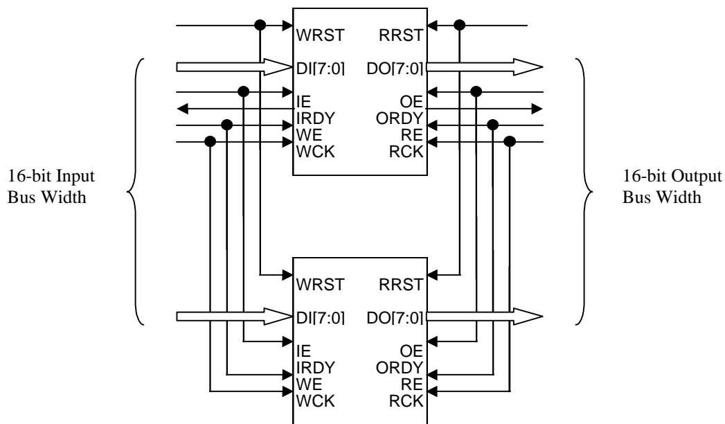
AL440B Data Bus Width Expansion
