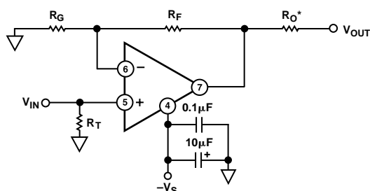
* R_O CHOSEN FOR CHARACTERISTIC IMPEDANCE. NONINVERTING CONFIGURATION
