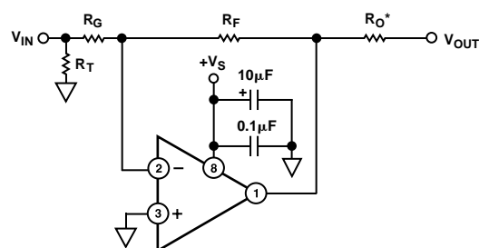
* R_O CHOSEN FOR CHARACTERISTIC IMPEDANCE. INVERTING CONFIGURATION
