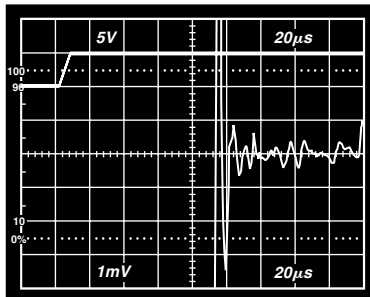
Figure 12c. Turn-On Settling
