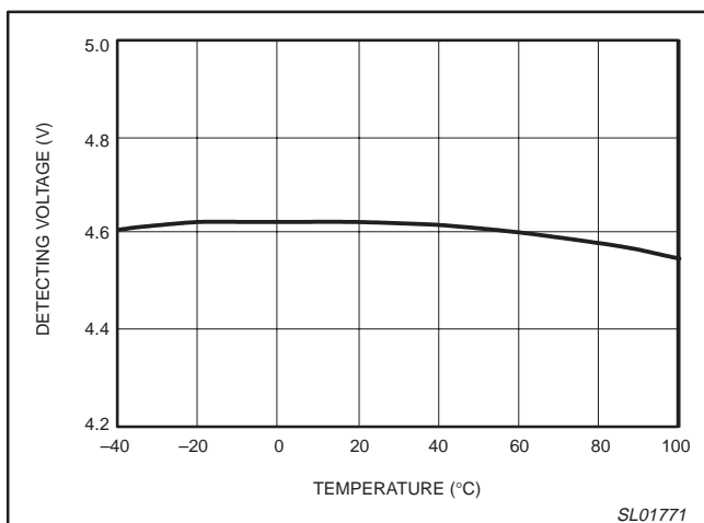
Figure 32. Detection voltage versus temperature.
