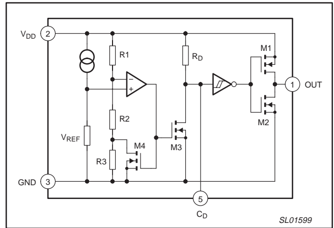
Figure 74. SA56616-XX equivalent circuit.
