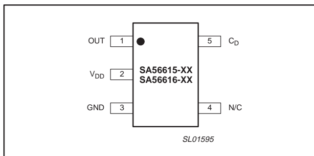
Figure 3. Pin configuration.
