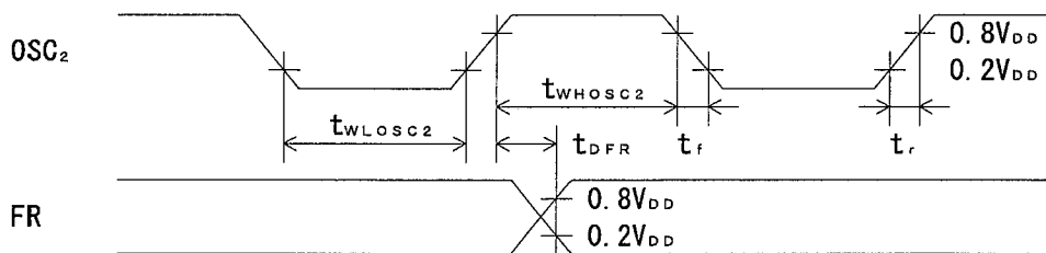
fig.5 Display control timing characteristics
