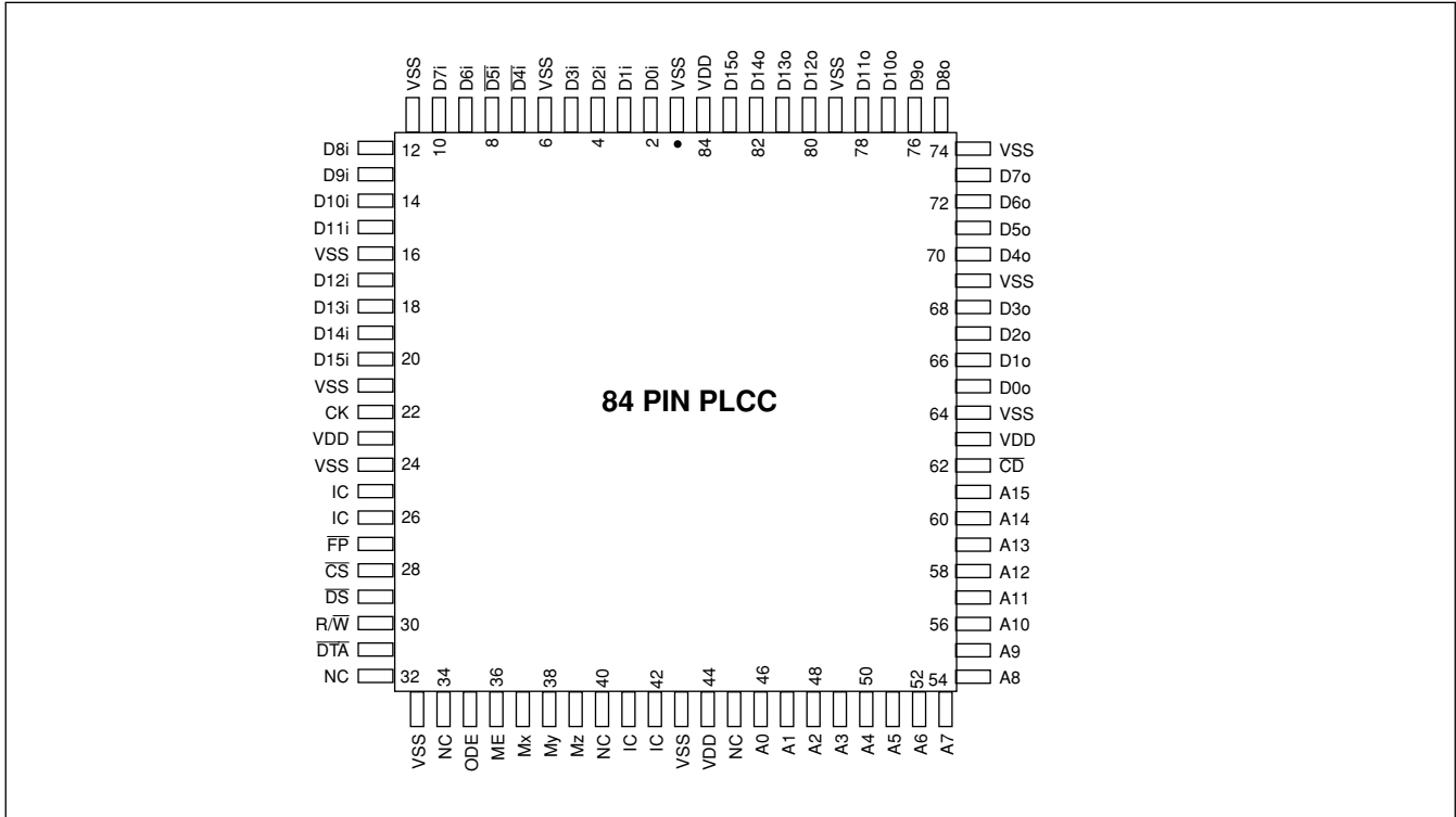
Figure 2 - Pin Connections
