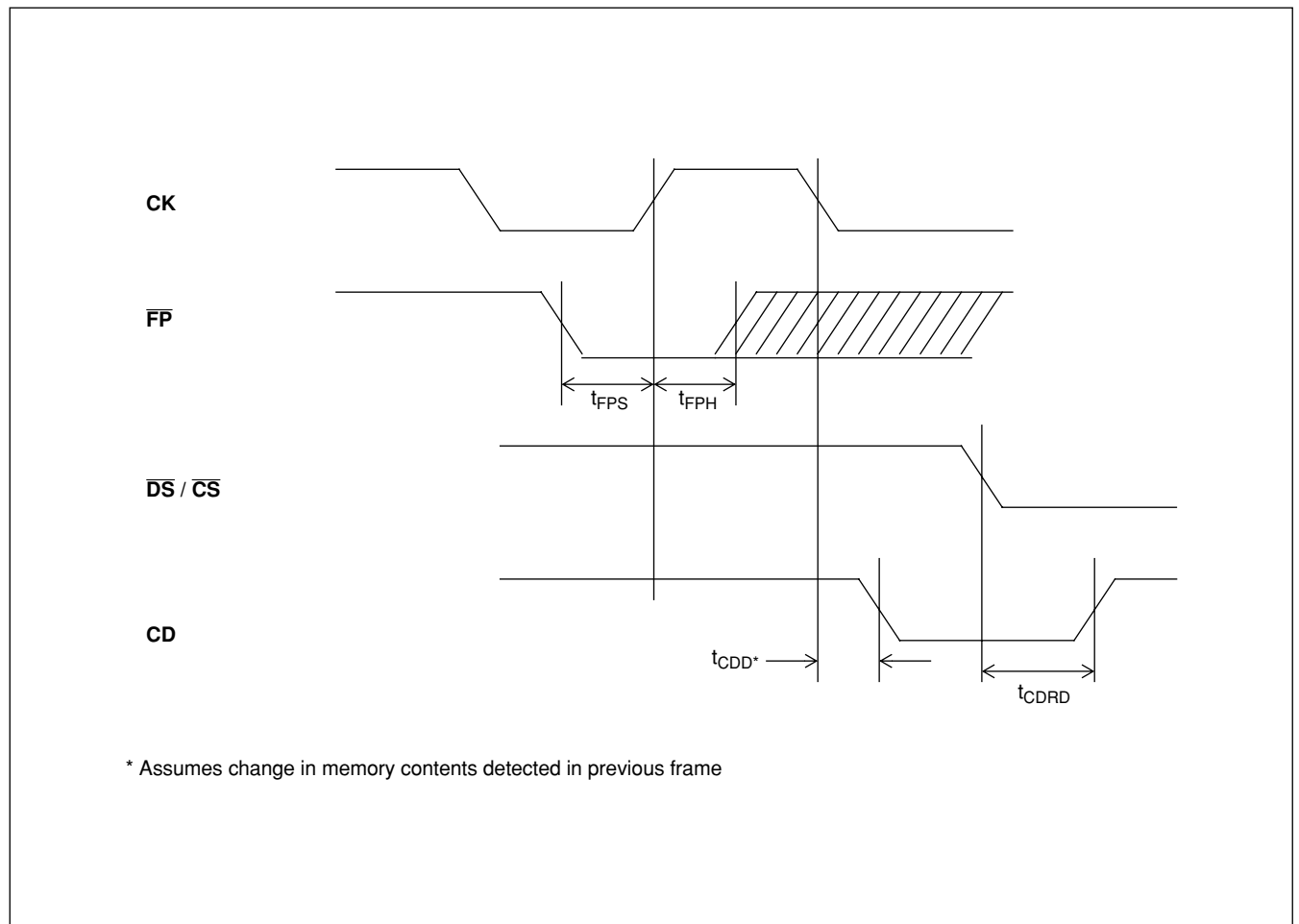
Figure 30 - Frame Pulse and Change Detect Timing
