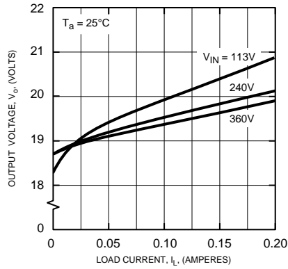
OUTPUT VOLTAGE - LOAD CURRENT CHARACTERISTICS
