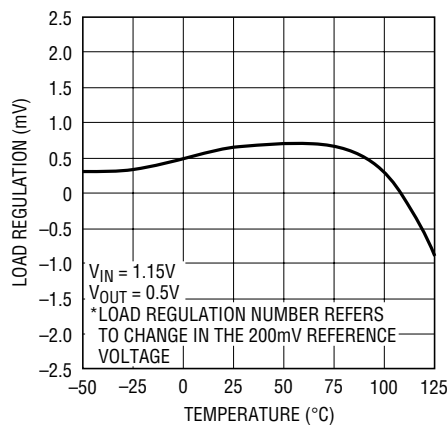
Load Regulation \Delta I_L = 1\text{mA to } 500\text{mA}
