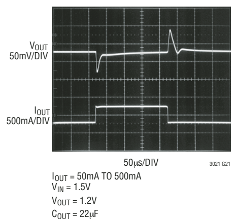
Transient Response
