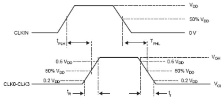
Figure 2. Voltage Thresholds for Propagation Delay ( t_{pd} ) Measurements
