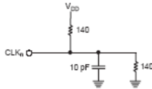
Figure 1. Test Load Circuit
