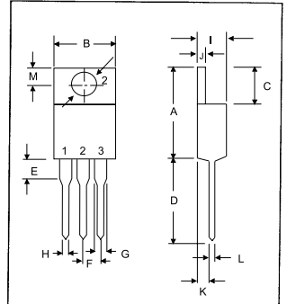
TO-220AB
