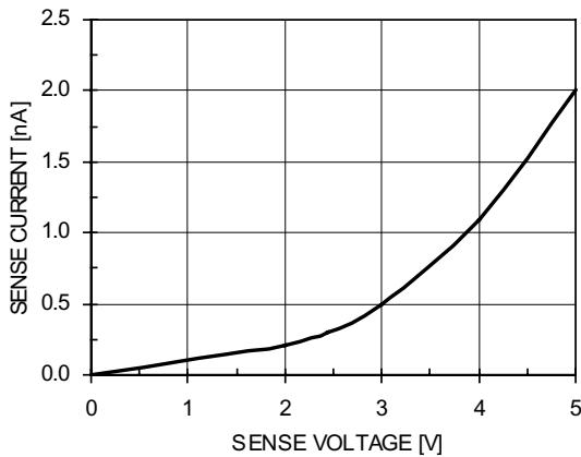
Sense Input Current vs. Voltage
