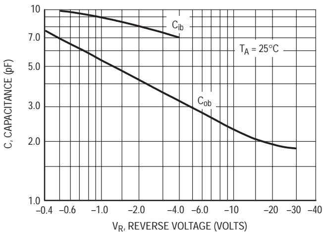
Figure 15. Capacitances
