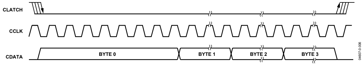
Figure 9. SPI Write format (Single-Write Mode)
