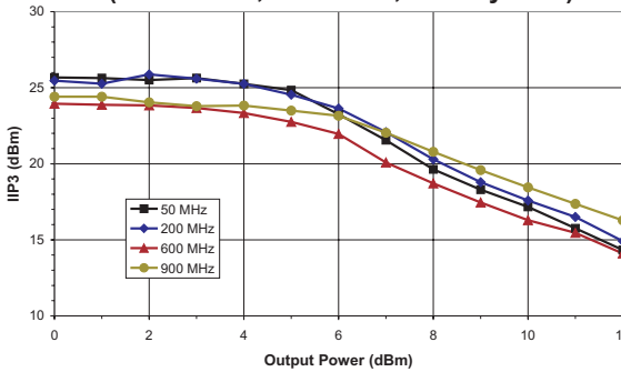
Figure 10: Input IP3 vs. Output Power (T A = +25 °C, V DD = +5 V, 75 Ω system)
