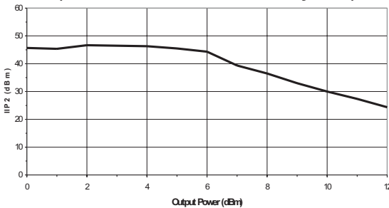
Figure 12: Input IP2 vs. Output Power (T A = +25 °C, V DD = +5 V, 75 Ω system)
