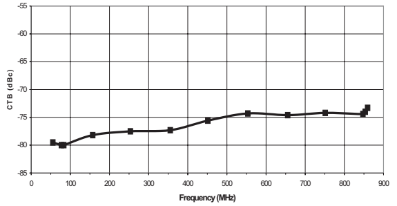
Figure 9: CTB vs. Frequency (T A = +25 °C, V DD = +5 V, 132 channels, +15 dBmV input power per channel)
