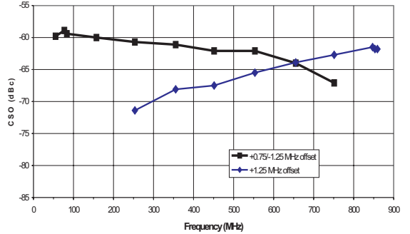
Figure 11: CSO vs. Frequency (T A = +25 °C, V DD = +5 V, 132 channels, +15 dBmV input power per channel)
