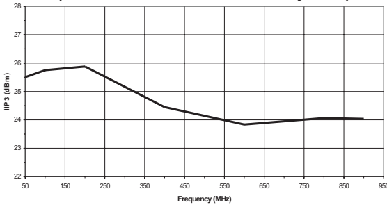
Figure 8: Input IP3 vs. Frequency (T A = +25 °C, V DD = +5 V, 75 Ω System)
