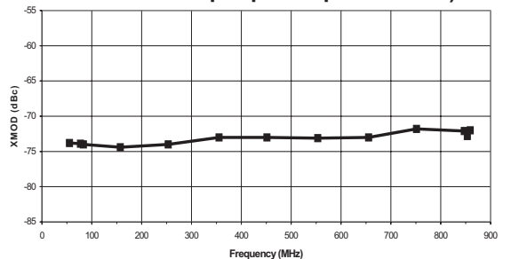
Figure 13: XMOD vs. Frequency (T A = +25 °C, V DD = +5 V, 132 channels, +15 dBmV input power per channel)
