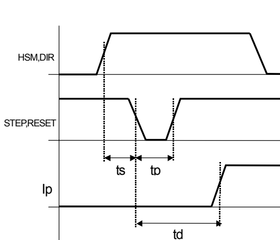
Fig.4 Timing chart
