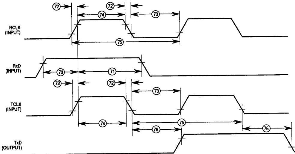
Figure 20. XPC Serial Data RxD, TxD, and Serial Clocks (RCLK, TCLK) Timing Diagram
