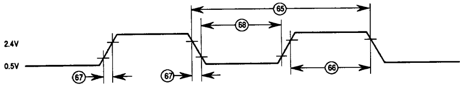
Figure 19. Clock (CLK) Timing Diagram
