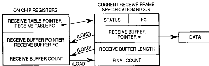
Figure 6. Receive Frame Specification Table
