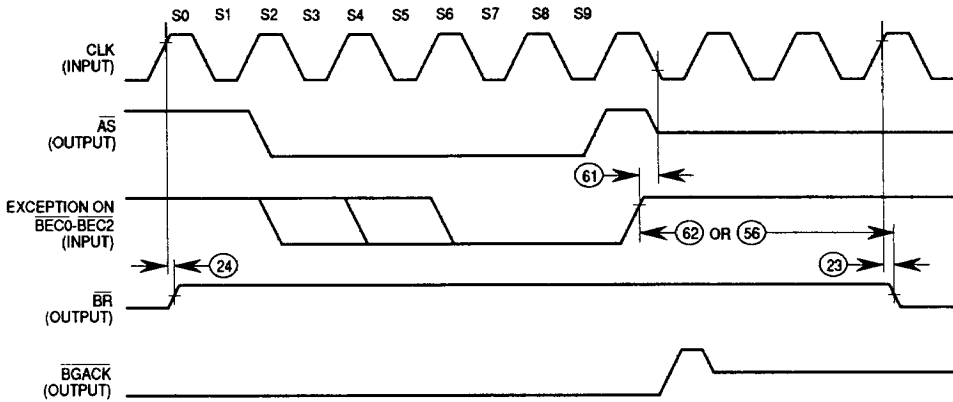
Figure 17. BR after Previous Exception Timing Diagram
