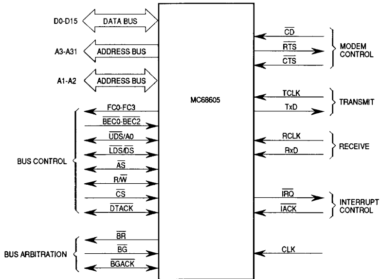
Figure 8. Functional Signal Groups
