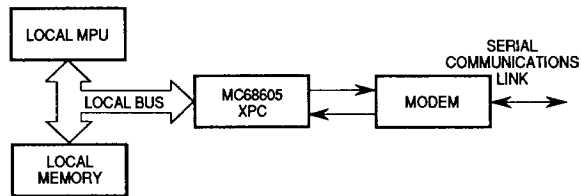
Figure 1. XPC System Configuration
