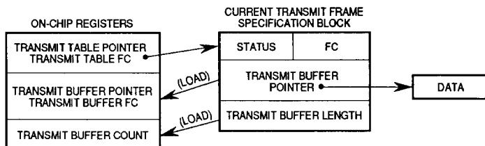
Figure 5. Transmit Frame Specification Table
