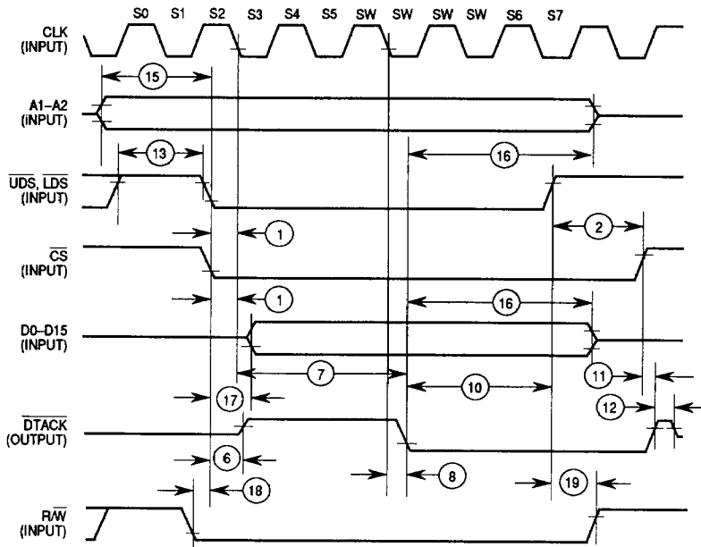
Figure 10. Host Processor Write Cycle Timing Diagram
