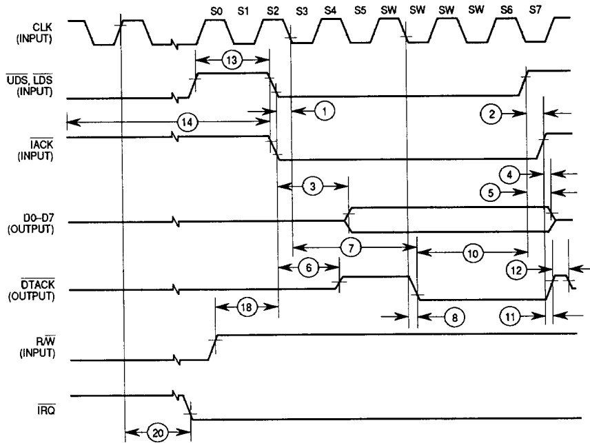
Figure 11. Interrupt Acknowledge Cycle Timing Diagram
