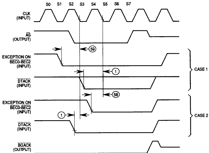
Figure 17. BR after Previous Exception Timing Diagram
