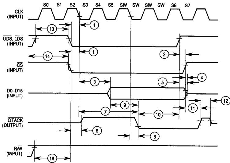
Figure 9. Host Processor Read Cycle Timing Diagram
