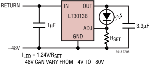
Constant Brightness for Indicator LED over Wide Input Voltage Range
