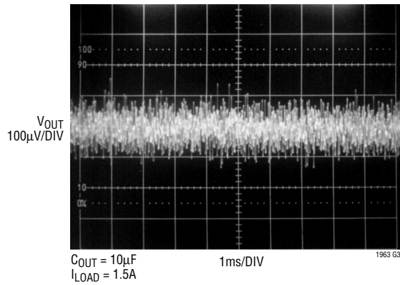
LT1963A-3.3 10Hz to 100kHz Output Noise
