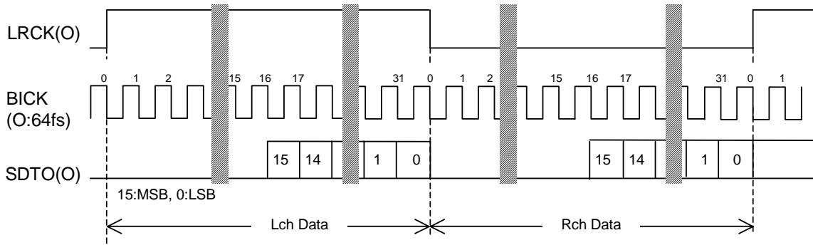
Figure 27. Mode 0 Timing
