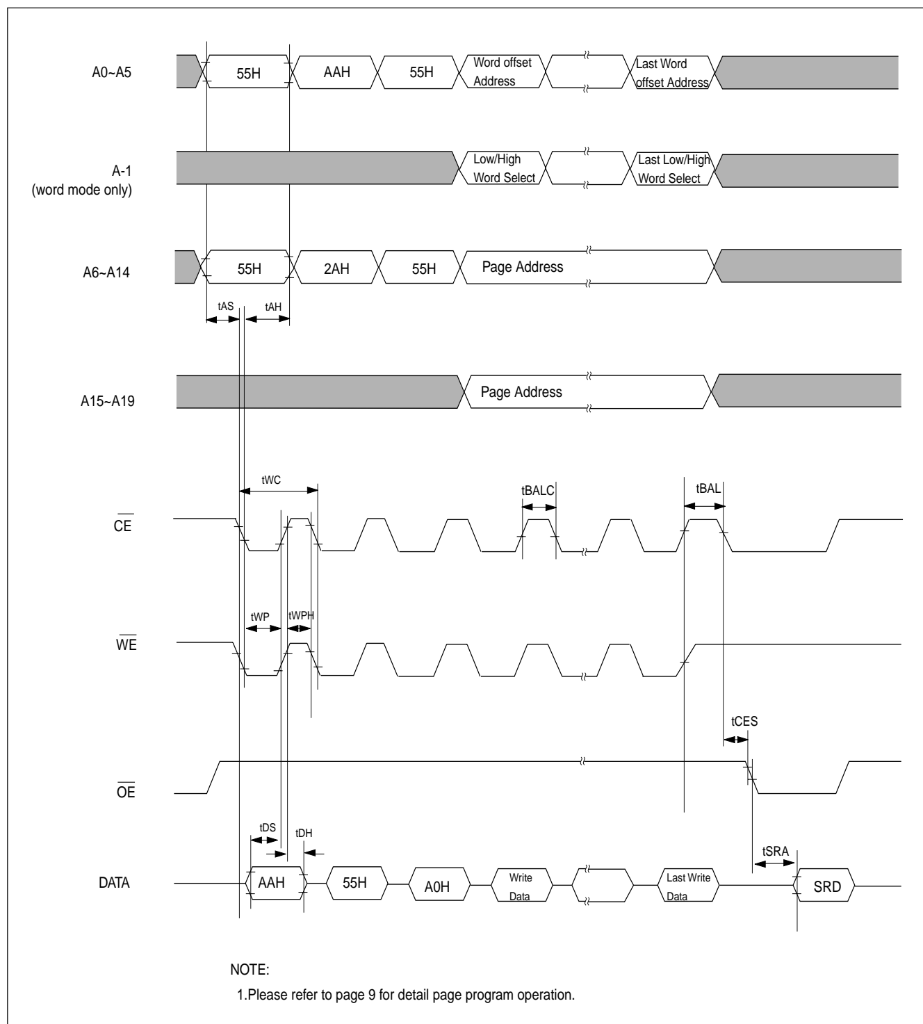
Figure 14. AUTOMATIC PAGE PROGRAM TIMING WAVEFORM(Alternate \overline{\text{CE}} Controlled)
