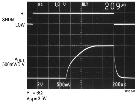
Output Voltage Soft-Start and Shutdown (LTC3250-1.5)
