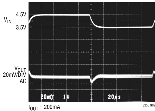
Line Transient Response (LTC3250-1.5)
