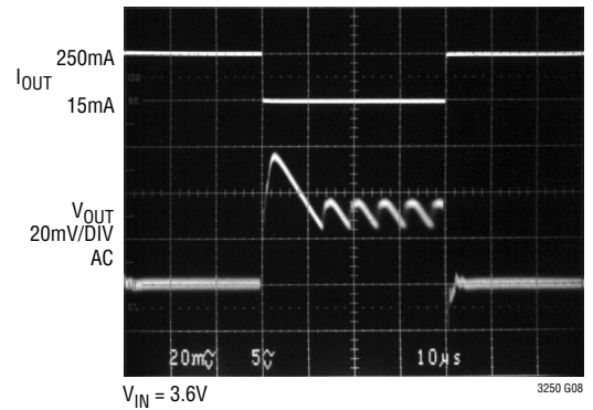
Output Current Transient Response (LTC3250-1.5)
