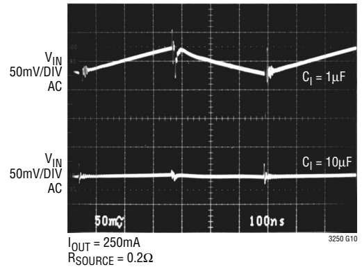
Input Voltage Ripple vs Input Capacitor (LTC3250-1.5)
