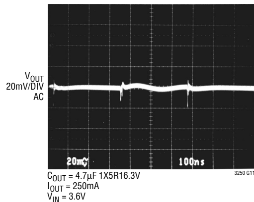
Output Voltage Ripple (LTC3250-1.5)
