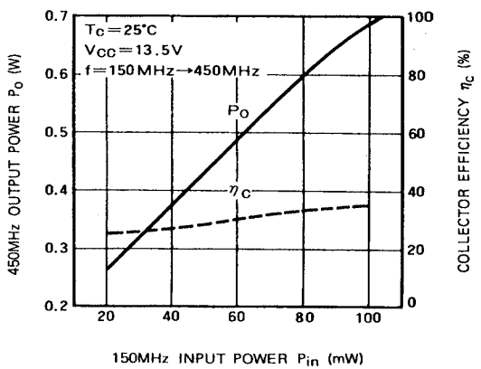
TRIPLER OUTPUT POWER, COLLECTOR EFFICIENCY VS. INPUT POWER
