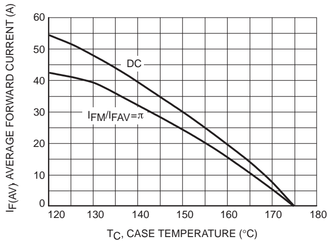
Figure 4. Current Derating
