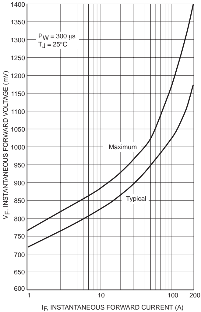
Figure 1. Forward Voltage
