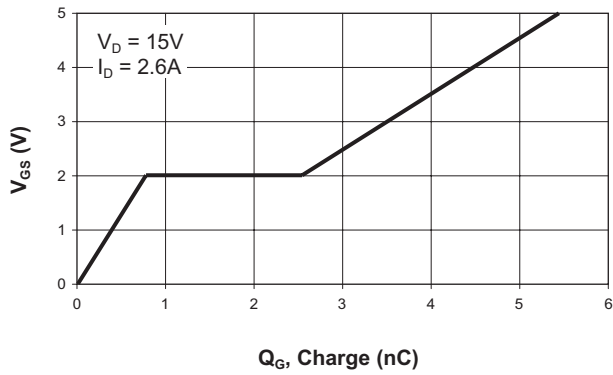
Gate Charge
