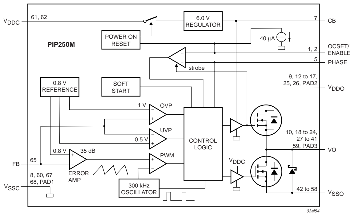
Fig 1. Block diagram
