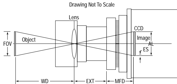
Figure 5. Optical Interface Diagram
