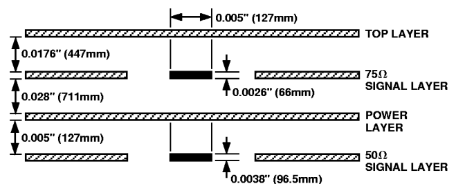
Figure 41. PCB Dimensions
