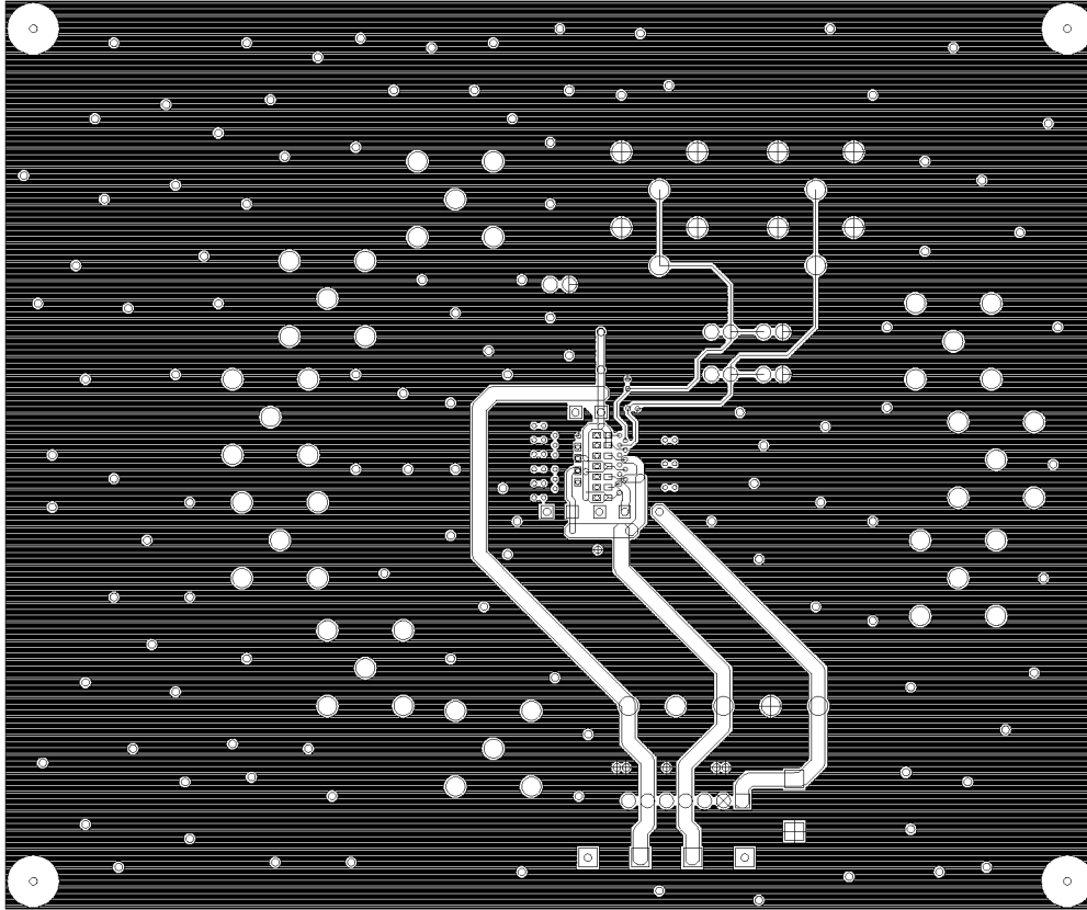
Figure 47. Board Layout (Circuit Side;) 50 Ω Signal Layer
