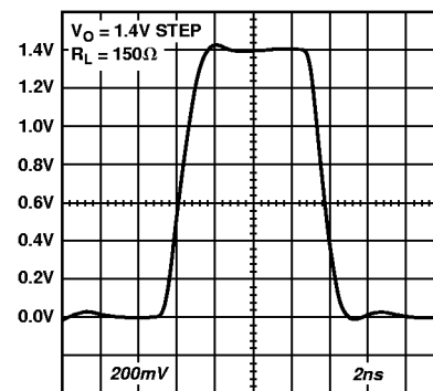
Figure 1. AD8185 Pulse Response; R L = 150 Ω
