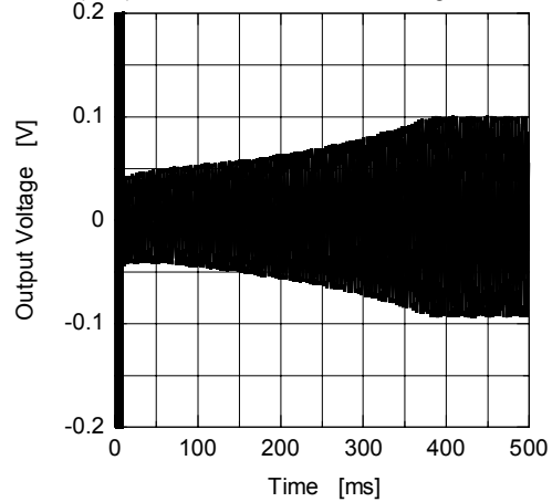
AGC Recovery Time (C:9pin=2.2 μF)
