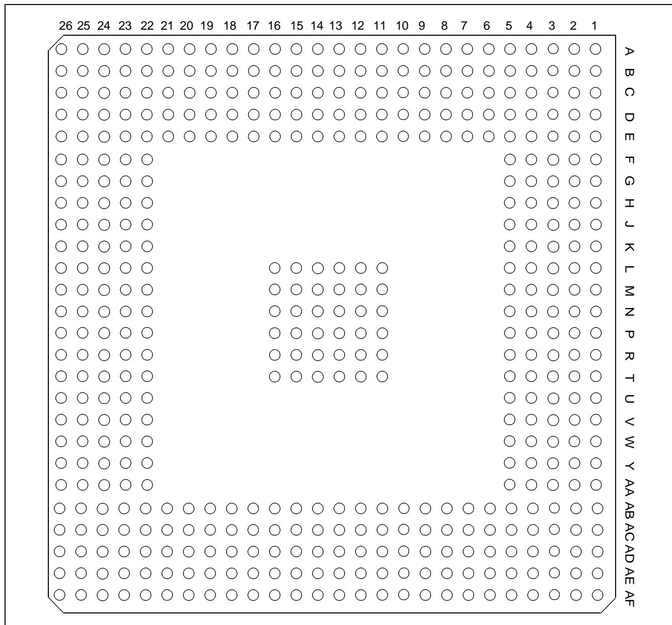
Figure 2 - 456 PBGA
