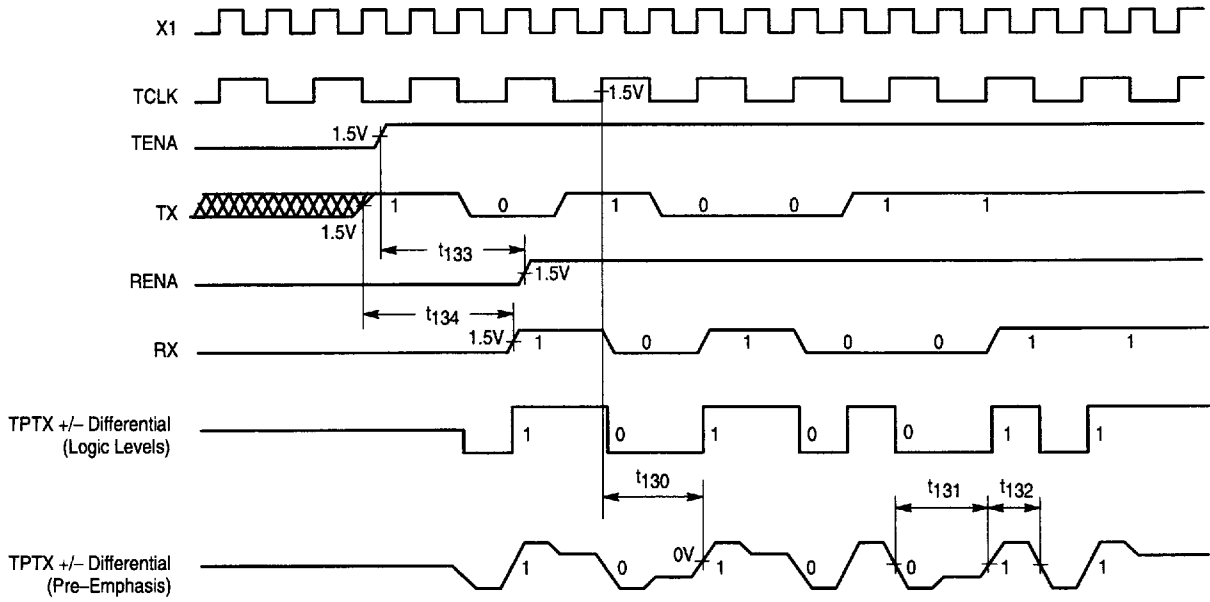
Figure 24. TPTX Transmit Timing (Start of Frame) Switching
