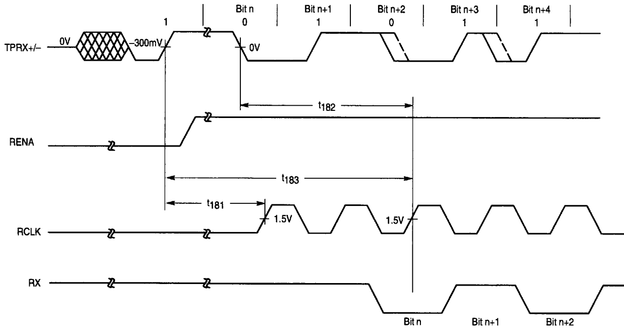
Figure 32. TPRX Receive Timing (Start of Frame)
