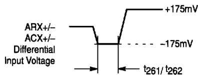
Figure 39. ARX/ACX Timing
