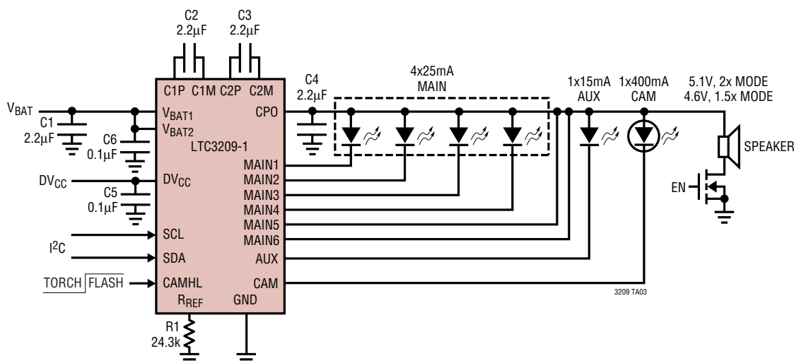
4 LED MAIN, 1 LED SUB, 400mA CAM LED Controller Plus Regulated Output
