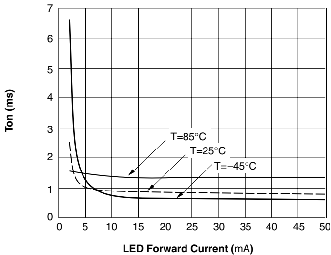
Figure 9. Turn-on Time vs. LED Current
