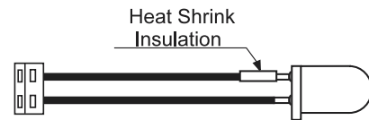
Custom LED with insulated leads and connector
