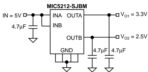
3.3V/2.5V Dual LDO
