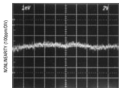
Gain Nonlinearity
