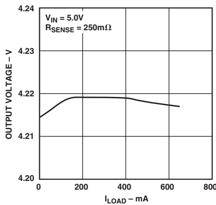
TPC 26. Charger V_{OUT} vs. I_{LOAD} ( V_{IN} = 5.0 V )
