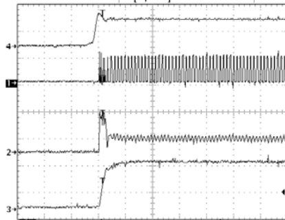
Figure 1: Fast V_{IN} Startup (Scope: 50\mu\text{s}/\text{div} )
