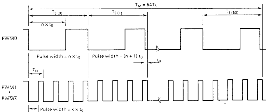
Figure 2-6. \overline{PWM} Output Waveform (It is shown to the additional pulse T_S(1) and T_S(63) of the \overline{PWM0} )
