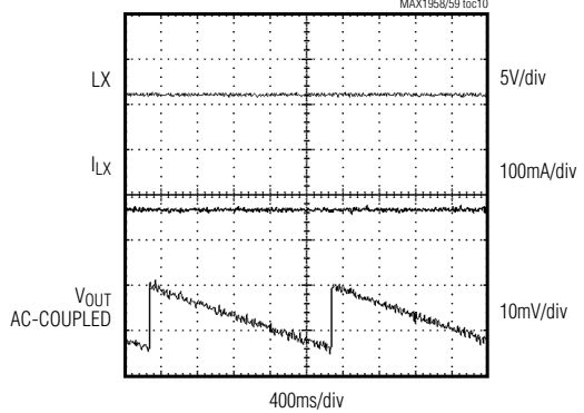
LIGHT-LOAD SWITCHING WAVEFORMS (PWM = AGND, I_{LOAD} = 30\text{mA} )
