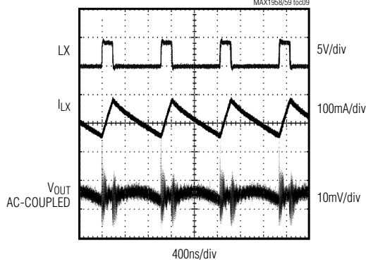
LIGHT-LOAD SWITCHING WAVEFORMS (PWM = IN, I_{LOAD} = 30\text{mA} )
