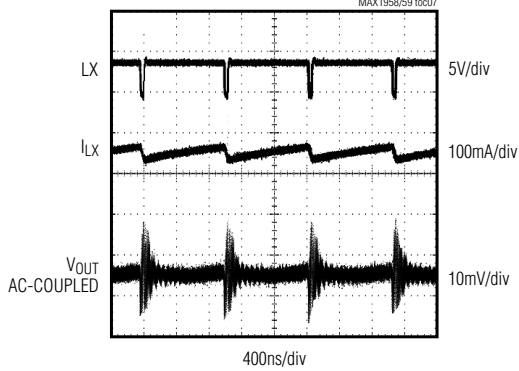
HEAVY-LOAD SWITCHING WAVEFORMS ( I_{LOAD} = 600\text{mA} )
