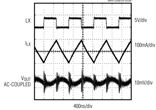
MEDIUM-LOAD SWITCHING WAVEFORMS ( I_{LOAD} = 300\text{mA} )
