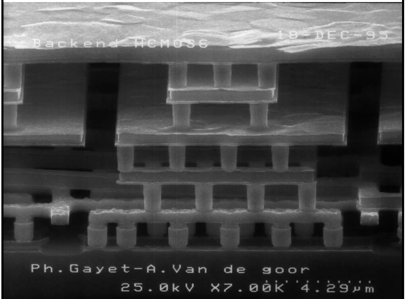
Figure 5 Evaluation Device Cross Section
