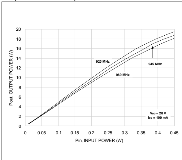
Output Power vs. Input Power PD57018
