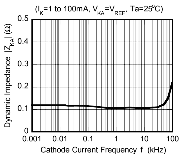
Dynamic Impedance
