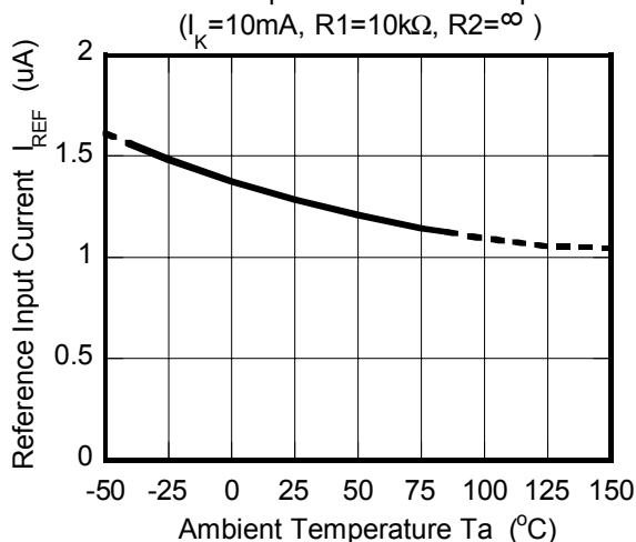
Reference Input Current vs. Temperature
