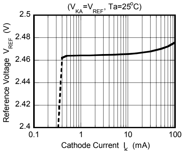
Reference Voltage vs. Cathode Current
