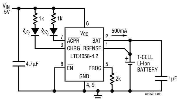
Full Featured Single Cell Li-Ion Charger
