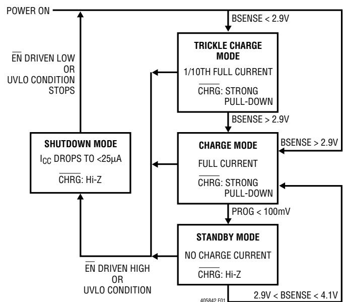
Figure 1. State Diagram of a Typical Charge Cycle
