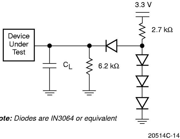
Figure 10. Test Setup
